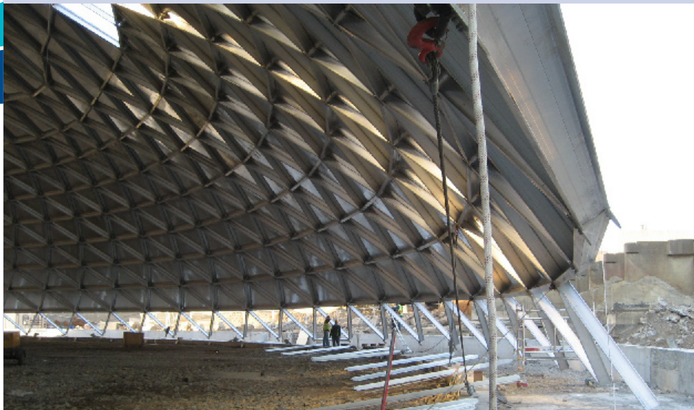
Irish Cement Plant, Platin - 5,000 sq. m - geodesic dome for materials storage.
